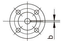
ROUND WITH KEY FOR SIZES 28" THROUGH 40"
