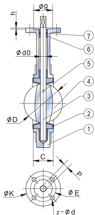
DIAGONAL SQUARE HEAD FOR SIZES 14" THROUGH 24"
