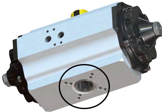
Typical Rack and Pinion Actuator mounting
