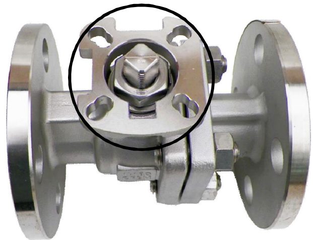
Typical Direct Mount Ball Valve Note: Choice of two ISO patterns
